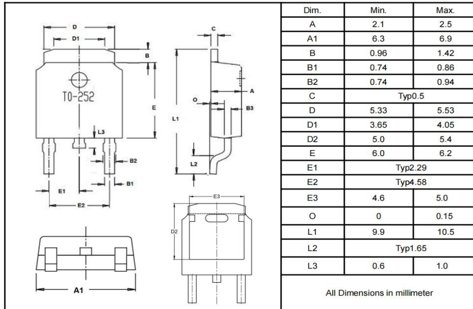
TO-252
