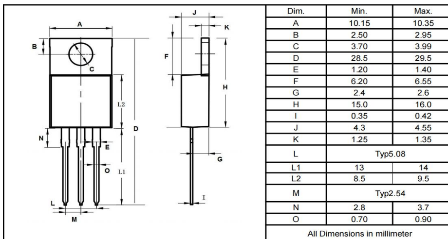
TO-220AB
