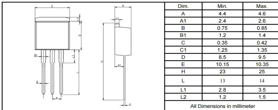
TO-262
